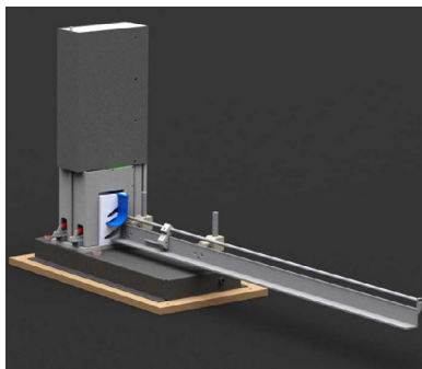
Scoop longitudinal cutter
