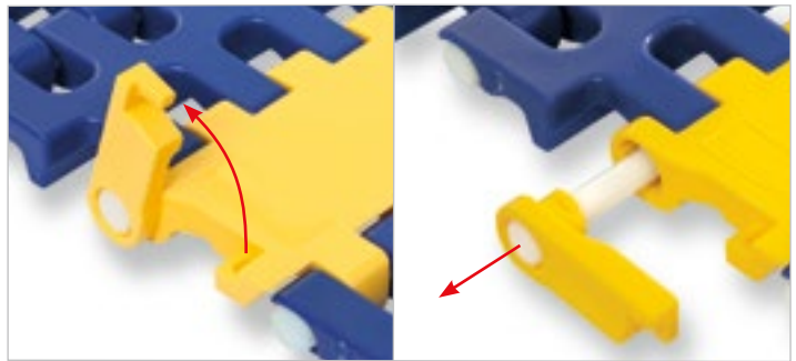
Lever system: 1" – 2" pitch system
