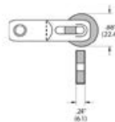
ROLLERS-XX-1-1/2
