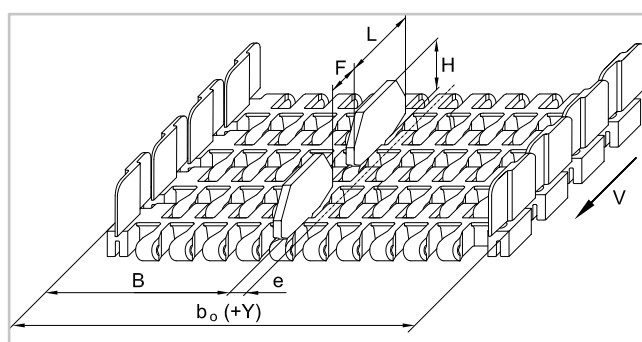
Lane divider
