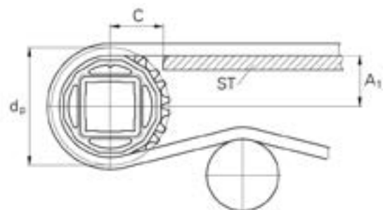
Molded sprocket
