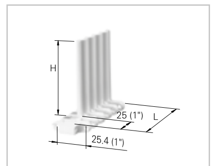
M253JF07, open hinge; indent flight, corrugated
