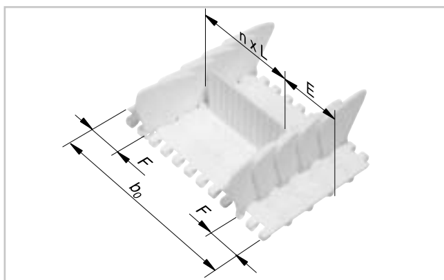
M2510 with flights M2510F05 and side guards
