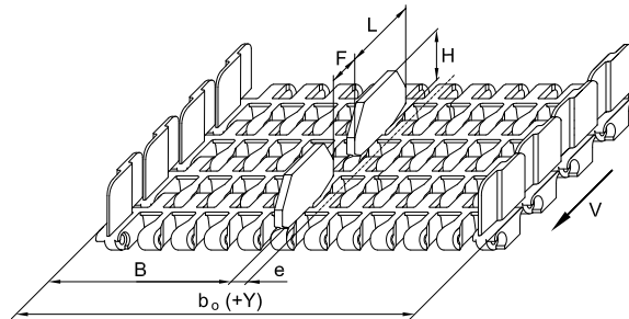
Lane divider
