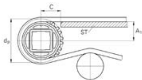
Molded sprocket
