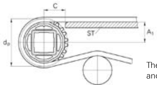
Molded sprocket
