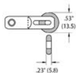
ROLLERS-XX-1/2
