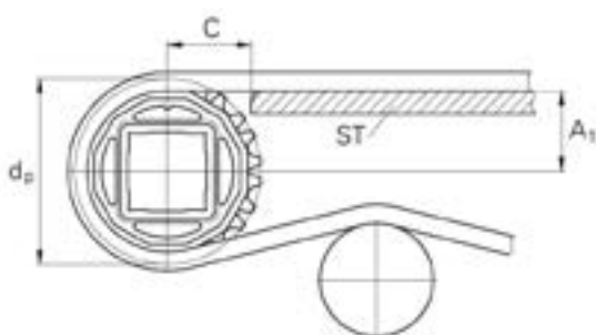
Machined sprocket
