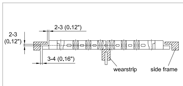
Side tabs M2544
