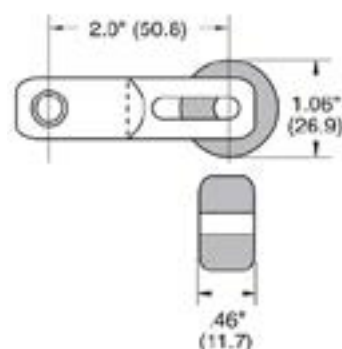
ROLLERS-XX-2
